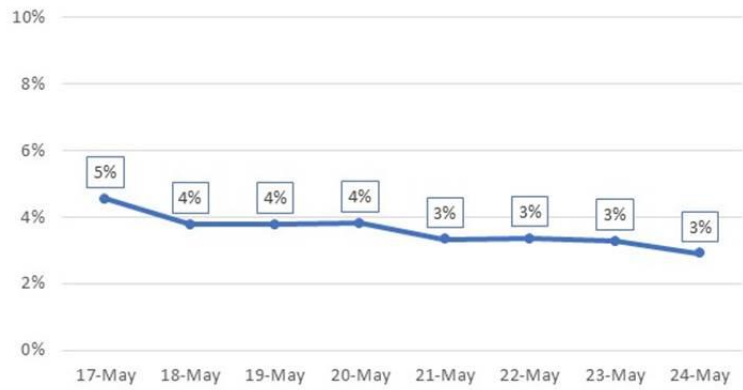
Test Volume: 3-Day Rolling Avg
