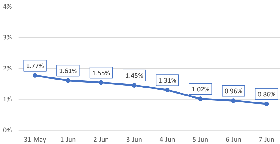
% New Test Positives: 7-Day Rolling Avg
